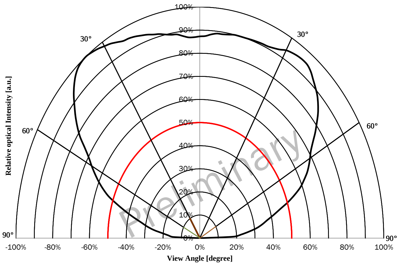
FIG 7. Far-field Emission Pattern
