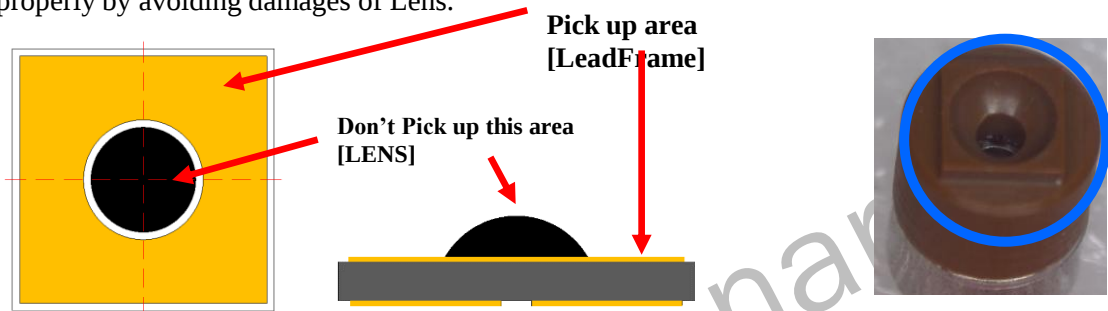
Figure 3(a). Pick up point of LED
