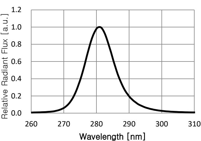
FIG 6. Typical Spectrum
